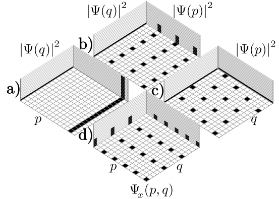
FIG. 4. The four classes of stabilizer states possible for odd non-prime d = 15 in terms of support: a) & b) maximally supported in p or q , c) maximally supported in p and q , and d) not maximally supported in p or q . The central grids denote the Wigner function |\Psi\rangle\langle\Psi|_x(p, q) for a stabilizer state \Psi with d = 15 . The projection of this state onto p -space is shown in the upper right ( |\Psi(p)|^2 ) and the projection onto q -space is shown in the upper left ( |\Psi(q)|^2 ).
