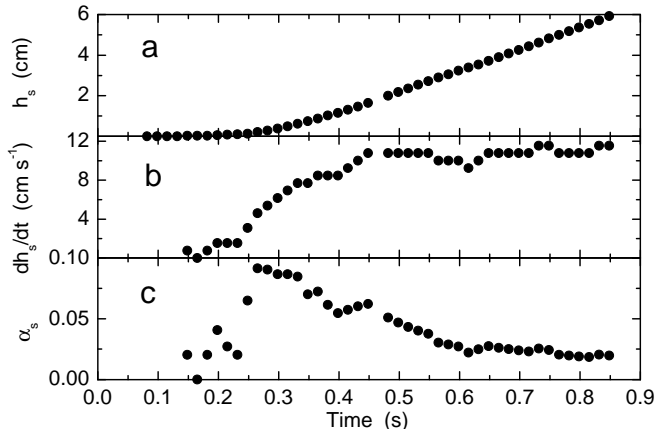
FIG. 4: Growth data vs. time for cell with wire of amplitude A_w = 0.3 cm. a ) the position of the front, b ) the velocity of the front, and c ) the instantaneous growth coefficient \alpha_s .
