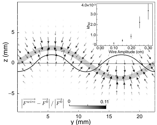
FIG. 3: Main figure: \left| \vec{F}^{wire} - \vec{F}^0 \right| / \left| \vec{F}^0 \right| in the midplane of the cell for A_w = 0.25 cm. Wide gray curve is projection of wire into the midplane, dotted line is fluid interface at t = 0 , and solid curve is actual fluid interface measured at t = 0.265 s. The force, which affects fluid 1 due to its large \chi_1 , is largest near the wire's crossing points, and results in a collection of fluid 1 at the crossing points. Inset: Dimensionless interface perturbation amplitude kh_{k0} vs. wire amplitude A_w .
