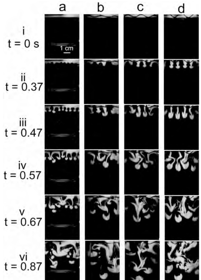
FIG. 2: Images of spike growth vs. time in sec., where t = 0 is the time at which the magnet current first begins to decrease. Column a) no wire; b – d) wires of amplitude A_w = 0.1, 0.2, and 0.3 \text{ cm} , respectively.
