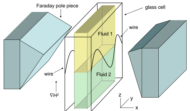
FIG. 1: Cartoon of experimental setup. Note that wires are attached to the outside of the cell, and that the x-axis view is expanded for clarity. The arrow indicating the direction of \nabla(H^2) applies only in the absence of the wires.
