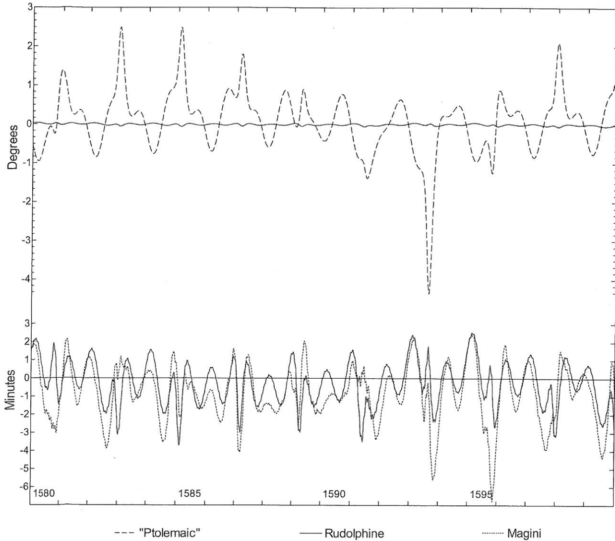
FIG. 5. Errors in geocentric longitudes of Mars. (Above) Ptolemaic calculation compared with Kepler's Rudolphine tables ; (below, at much enlarged scale) the Rudolphine errors compared with those from Magini's "Keplerian" method in his Supplementum ephemeridum .
