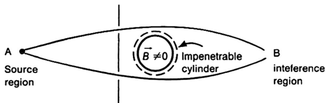
FIG. 1. Double-slit experiment illustrating the AB effect. Given the possible electron paths from source at A to detector at B , the resulting interference pattern changes as the \mathbf{B} in the impenetrable cylinder is turned on or off. Figure reproduced from J. J. Sakurai's Modern Quantum Mechanics .
