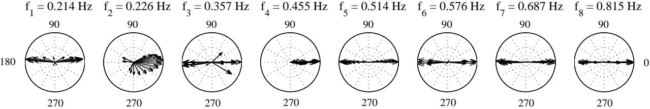
Fig. 10. Polar plot representation of vibration mode shapes identified using SSI-DATA
