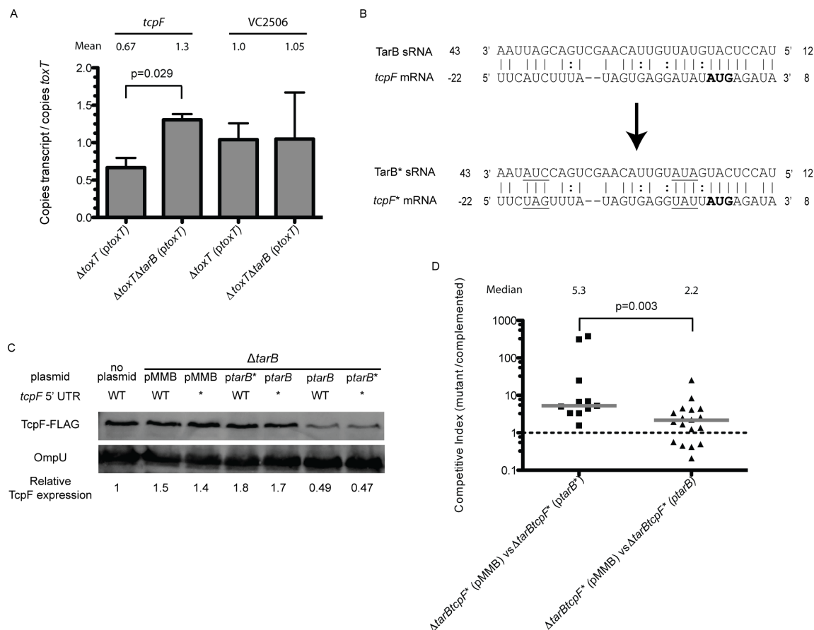
Figure 2.6: TarB interaction with the 5' UTR of tcpF .
