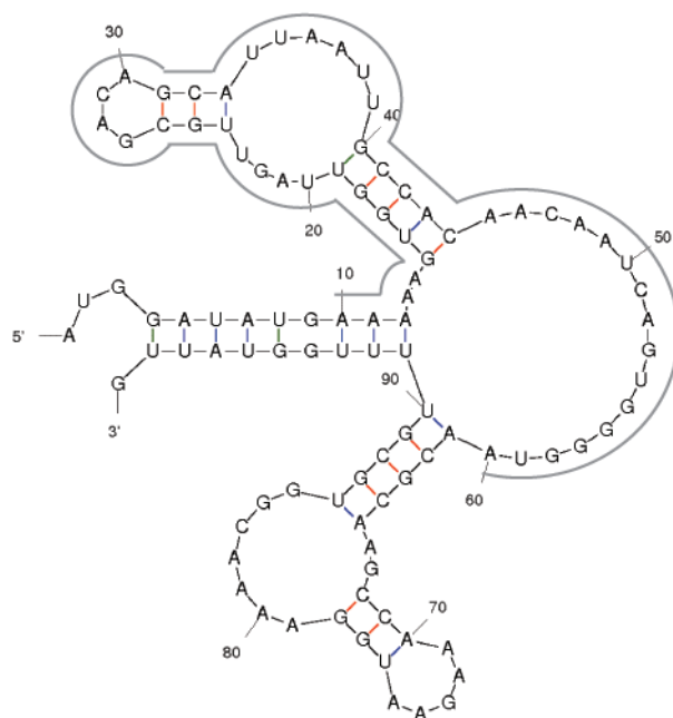
Figure 4.4 Mfold diagram of 5' region of VC1863 mRNA
