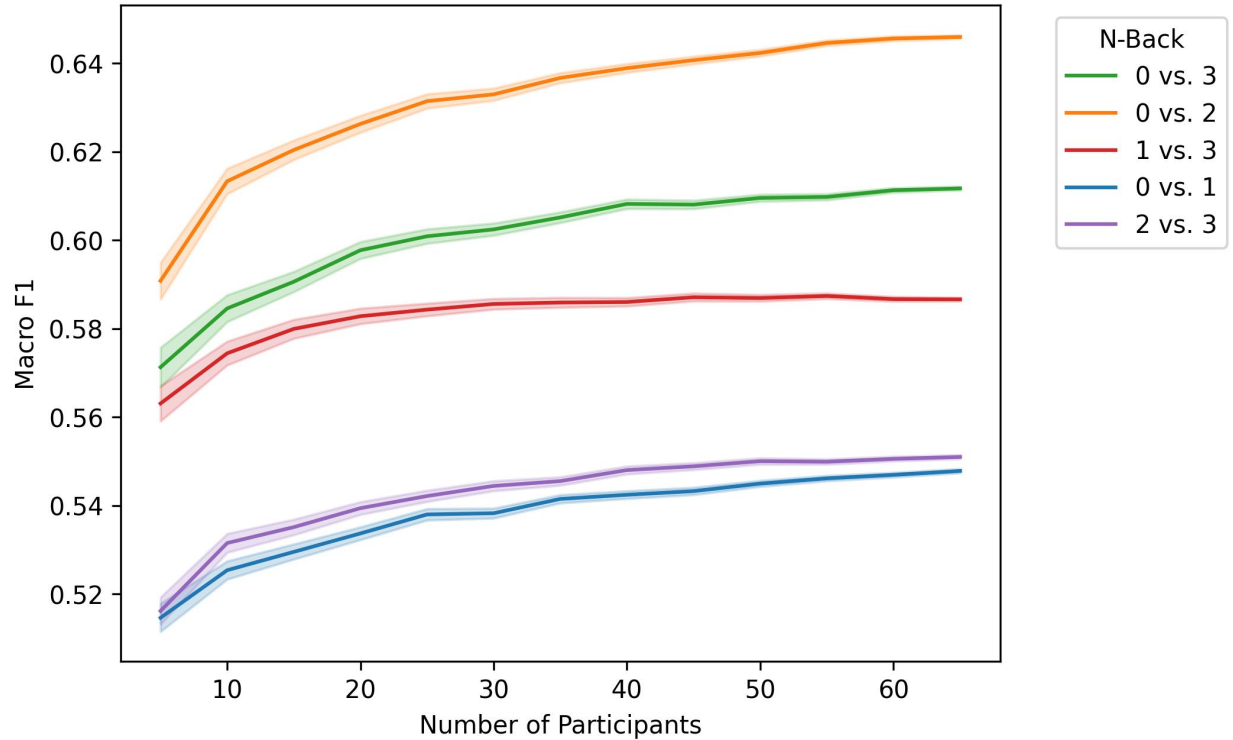
Figure 11.2: Analysis of LOO-CV RF runs across levels of N-Back comparison. For each number of participants to be used in the training set (x axis), 1000 models were used with a random set of this many participants taken from the total dataset; the y-axis displays the grand average over the 1000 LOO-CV result averages for each number of participants.
