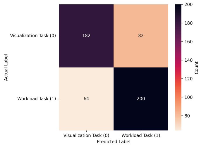
Figure 7.8: Confusion matrix for the best performing model from the LOO-CVV data when using limited probe sets: RF, which achieved 0.723 at a window size of 150 when using data only from the right probe locations. As seen in the confusion matrix for the all-probe data, proportions of classifications of both visualization and workload were similar, however in this case the workload task was correctly classified more often (200) than the visualization task (182), and workload was more often incorrectly classified (82) than visualization (64). Note that, given that the window size is half of that in Figure 7.6, the sample size is approximately double. In fact it is slightly larger, given that one extra sample could be gathered per-trial with this smaller window size.
