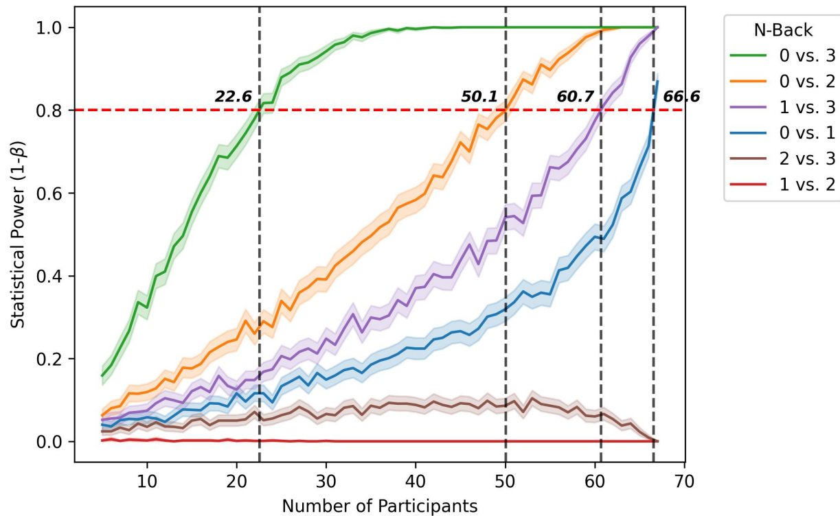
Figure 11.1: Power analysis of LLM results across levels of N-Back comparison. For each number of participants on the x axis, 1000 models were used with a random set of participants taken from the total dataset. The y-axis indicates the proportion of significant results at that level.
