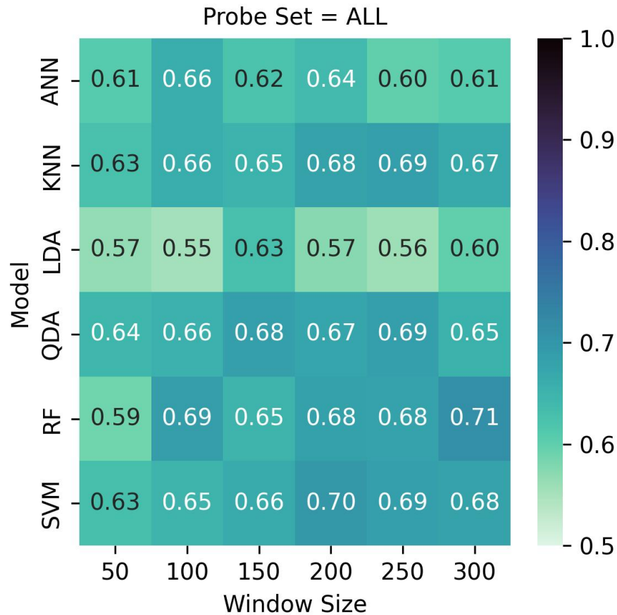
Figure 7.5: LOO cross validation results. Test set scores are produced based on the best model per-participant after inner hyperparameter optimization. Although RF with a window size of 300 performed best with 71%, it showed similar results across multiple window sizes. QDA, KNN, and SVM likewise performed well overall.
