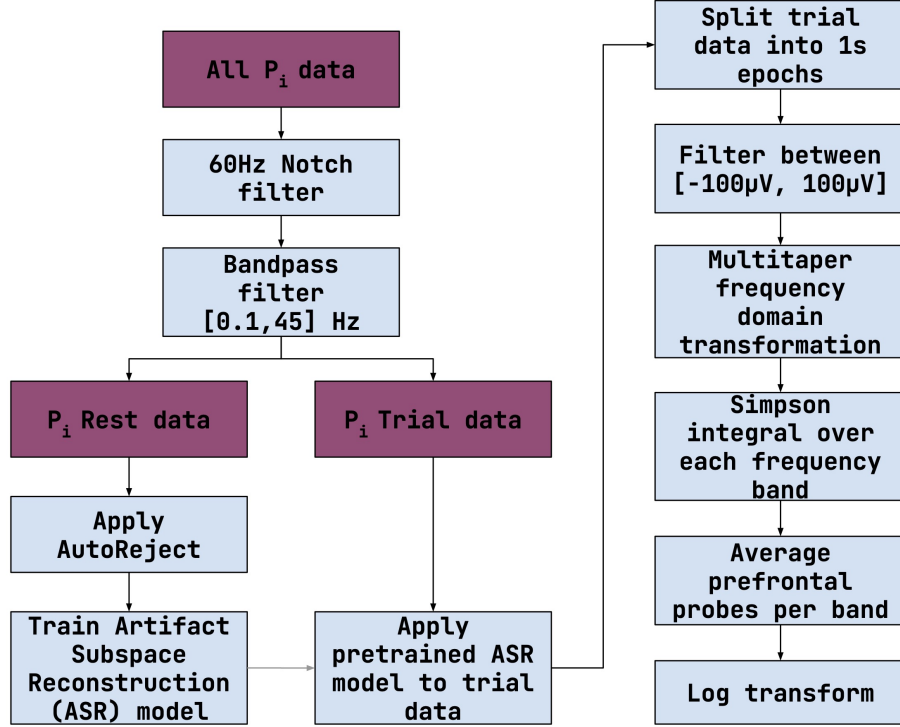
Figure 10.8: Visualization of the EEG processing pipeline showing data flow from raw signal through filtering, artifact removal, and spectral analysis stages for a single participant P_i . Rest data is cleaned with the AutoReject algorithm, and the cleaned data is used to train an ASR model, which is then applied to trial data before frequency domain transformation and averaging.
