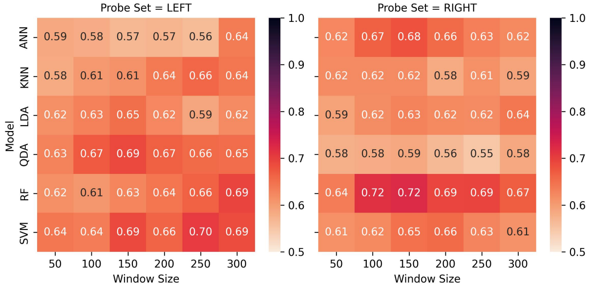
Figure 7.7: Performance comparison of models across window sizes using left and right probe sets, showing F1-scores for task classification. The heatmaps reveal distinctions in performance across probes for some models, with particular increases in performance for RF at lower window sizes for the right probes, whereas SVM performed notably better using the left probes' data at higher window sizes.
