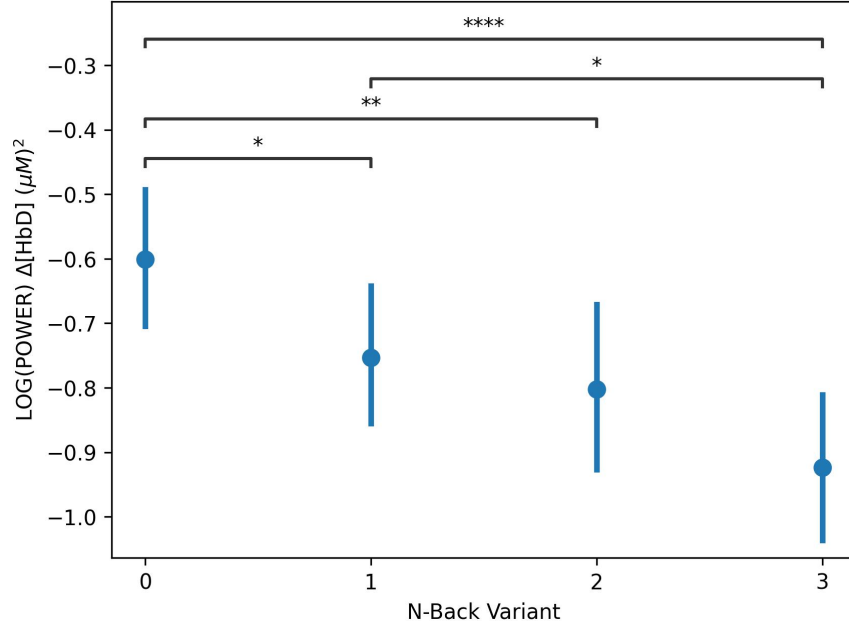
Figure 2.3: Log total power of \Delta[\text{HbD}] in the VLFO band in the left lateral PFC as a function of N-Back level. The increase of N-Back level, corresponding with an increase in left lPFC function (and mental workload), results in a significant decrease of total power in the VLFO band. Note that, although many pairs of N-Back tasks are differentiable in this way, not all are significant (e.g. 1 vs. 2, 2 vs. 3) 34 .
