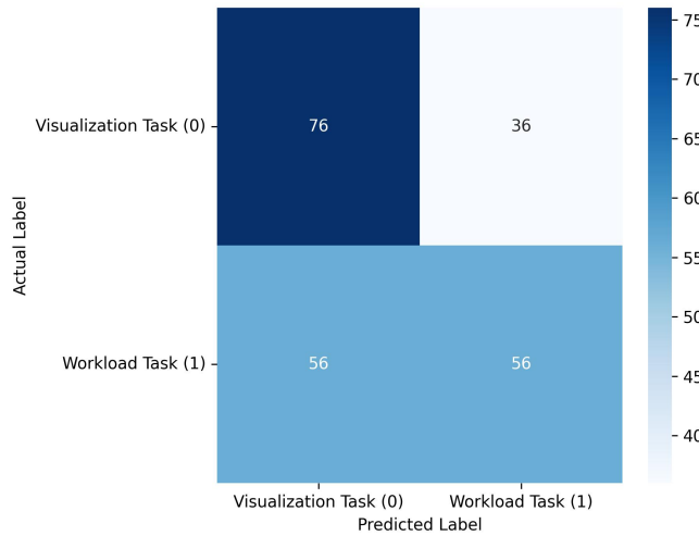
Figure 7.4: Confusion matrix across all participant predictions in the real-time experiment. Although the model classified a relatively high number of 76 visualization tasks correctly, it struggled to correctly identify workload tasks with only 56 correct classifications. Likewise, it incorrectly classified 56 workload samples as visualization and 36 visualization samples as workload. These results suggest that the model is not capable for usable real-time classification.
