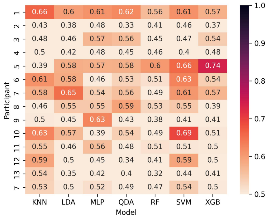
Figure 9.2: Machine learning scores per-participant across models. Darker boxes indicate higher scores. Although classification overall is not superb, variability across models and participants indicates potential application spaces may exist within such data.
