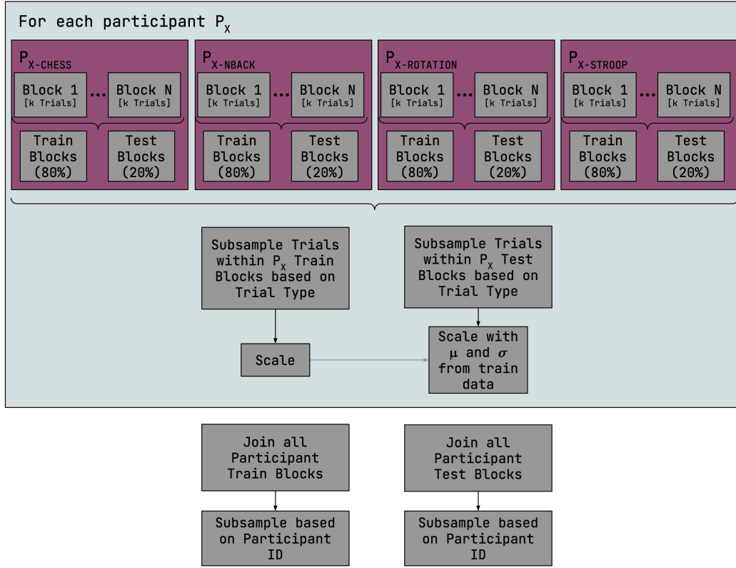
Figure 10.10: Visualization of one iteration of the data splitting steps for the Monte Carlo pipeline for cross-task classification. Blocks of grouped trials within each trial type for each participant are split into training and testing blocks randomly, with 80% of blocks in training and the remaining 20% of blocks in testing. All such training and testing blocks are combined for a given participant, and trials within the training and testing blocks are then subsampled (separately) to the lowest frequency label, and scaled. All such training and testing blocks for all participants and trial types are combined into single train and test sets, which are separately subsampled to the lowest frequency participant ID. F1 results are reported from both the precision and recall scores on the test set overall, and per-participant.
