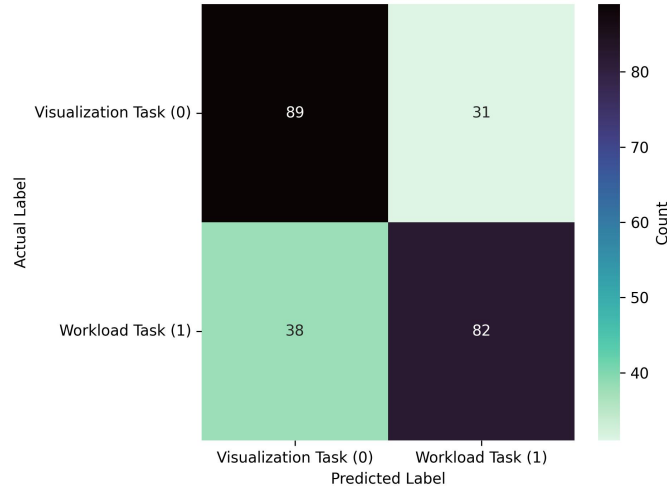
Figure 7.6: Confusion matrix for the best performing model from the LOO-CVV using all probes: RF, which achieved .710 at a window size of 300. The model predicted visualization and workload similarly well, correctly predicting 89 visualization samples, and 82 workload samples. The matrix also reveals relatively balanced misclassification patterns, with 31 visualization tasks misclassified as workload and 38 workload tasks misclassified as visualization.
